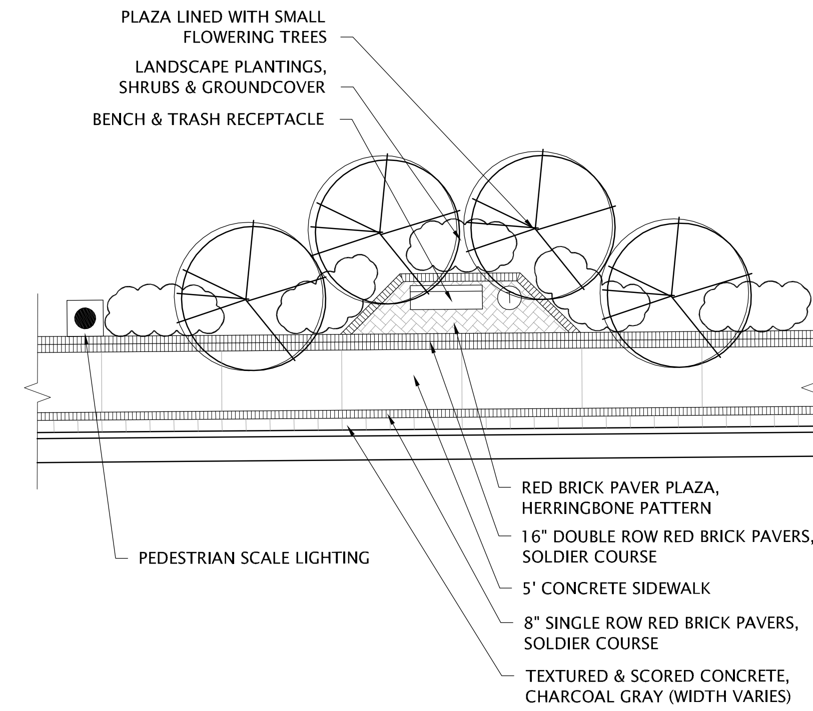
2 BUS STOP PLAZA Scale: 1/8" = 1'-0"
