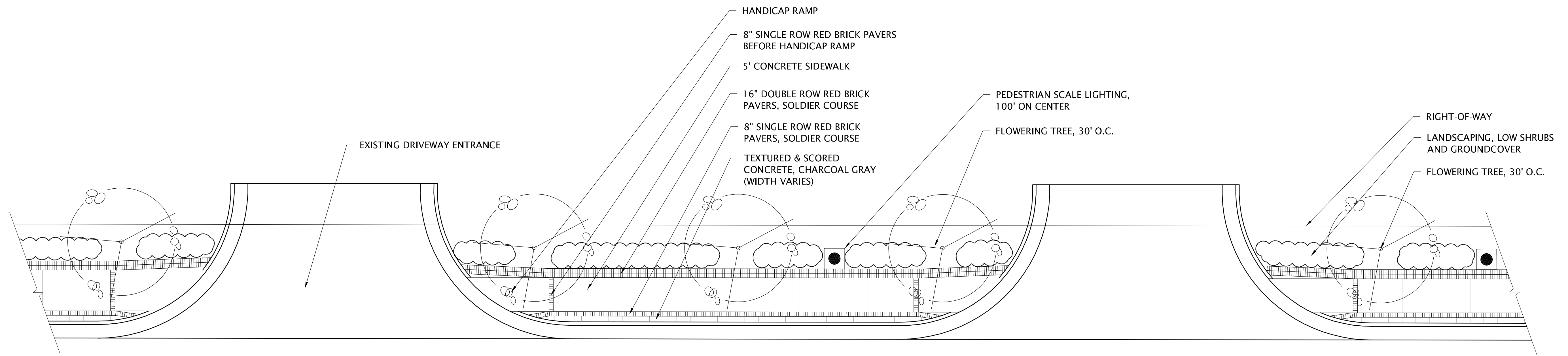
3 TYPICAL STREETSCAPE PLAN Scale: 1/8" = 1'-0"
