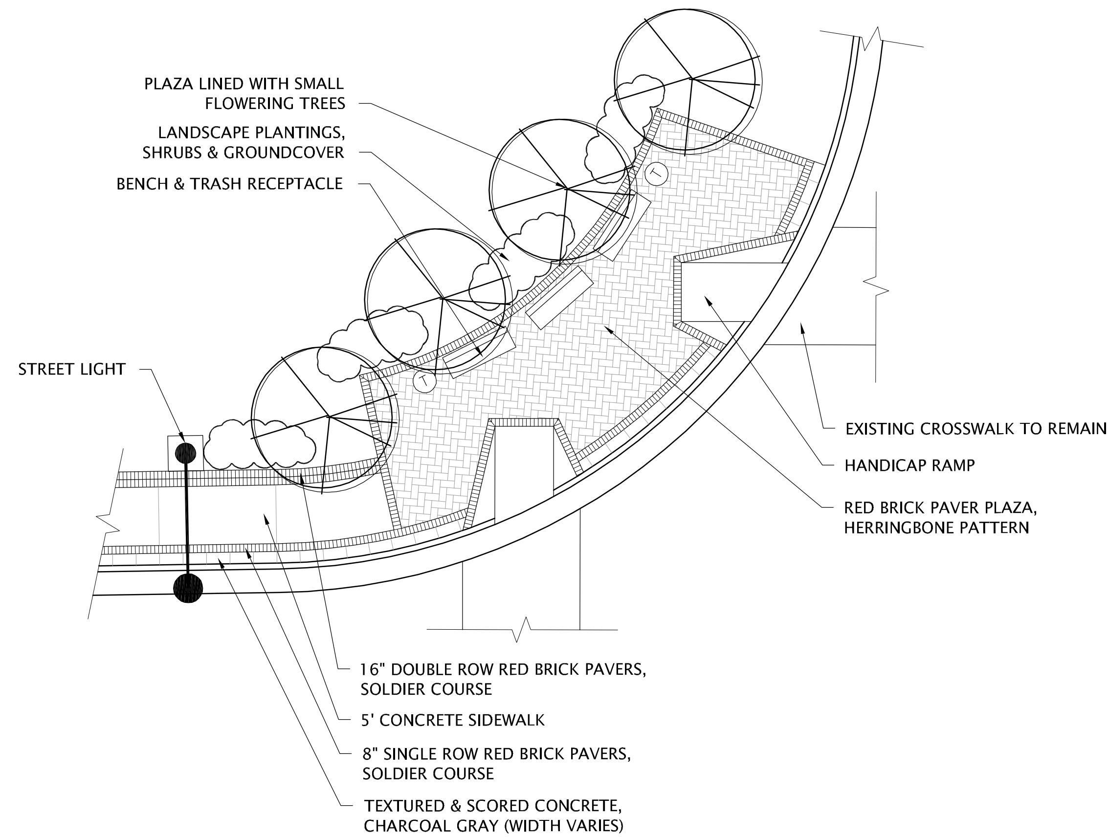
1 TYPICAL MAJOR INTERSECTION PLAZA Scale: 1/8" = 1'-0"
