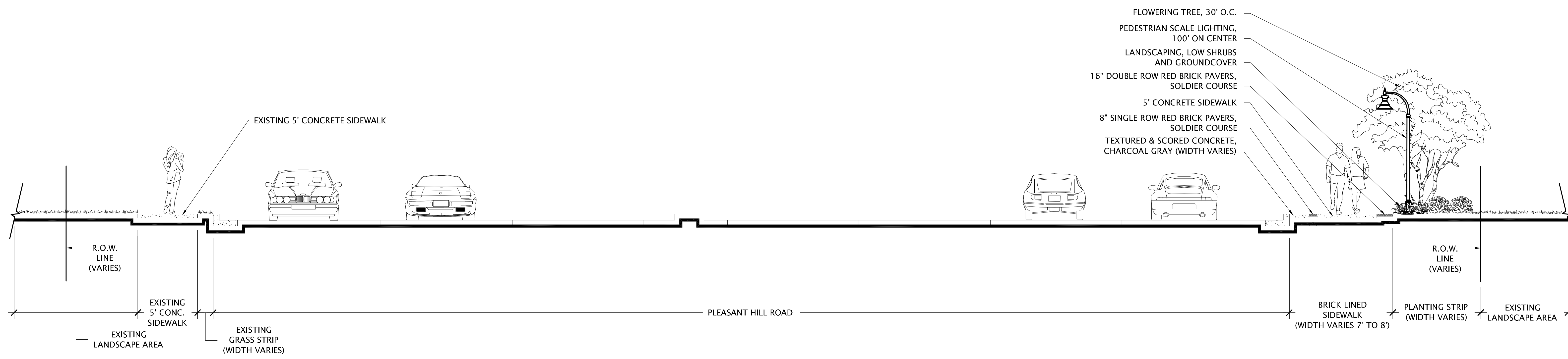
TYPICAL STREETSCAPE SECTION
